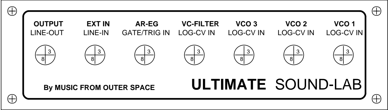
REAR WIRING VIEW OF SOUND LAB ULTIMATE AUXILLIARY PANEL SHOWING PCB CONNECTION POINTS
