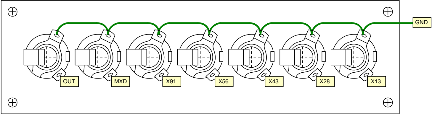
REAR WIRING VIEW OF SOUND LAB ULTIMATE AUXILLIARY PANEL SHOWING PCB CONNECTION POINTS
